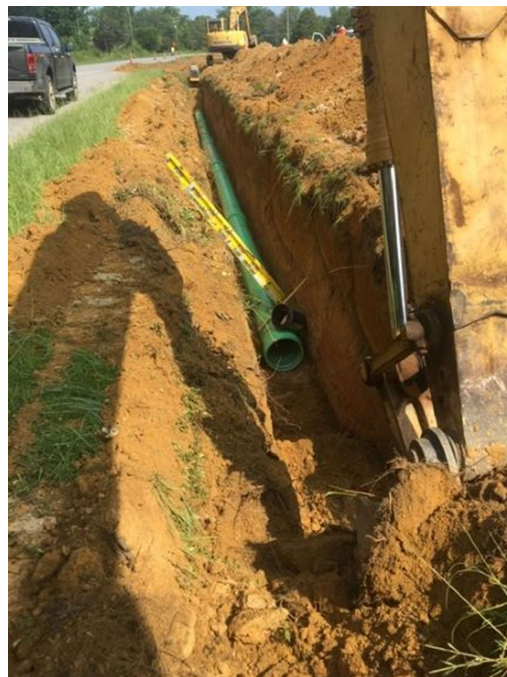
Photo 1: Pipeline install
