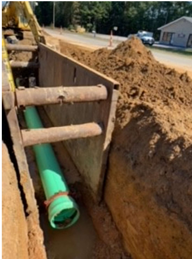
Photo 2: Line install
